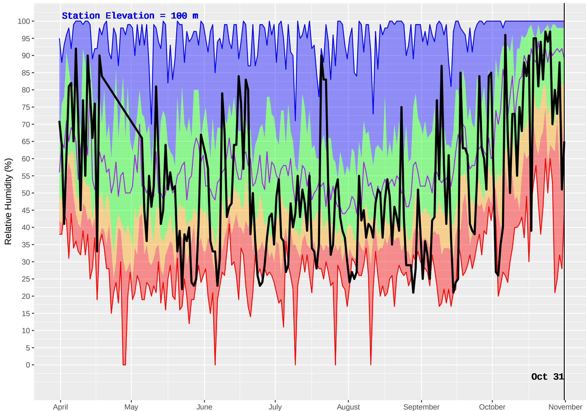
BEAVER CREEK (37) : Historical (1987–2016) and Current (2017) Noon Relative Humidity
