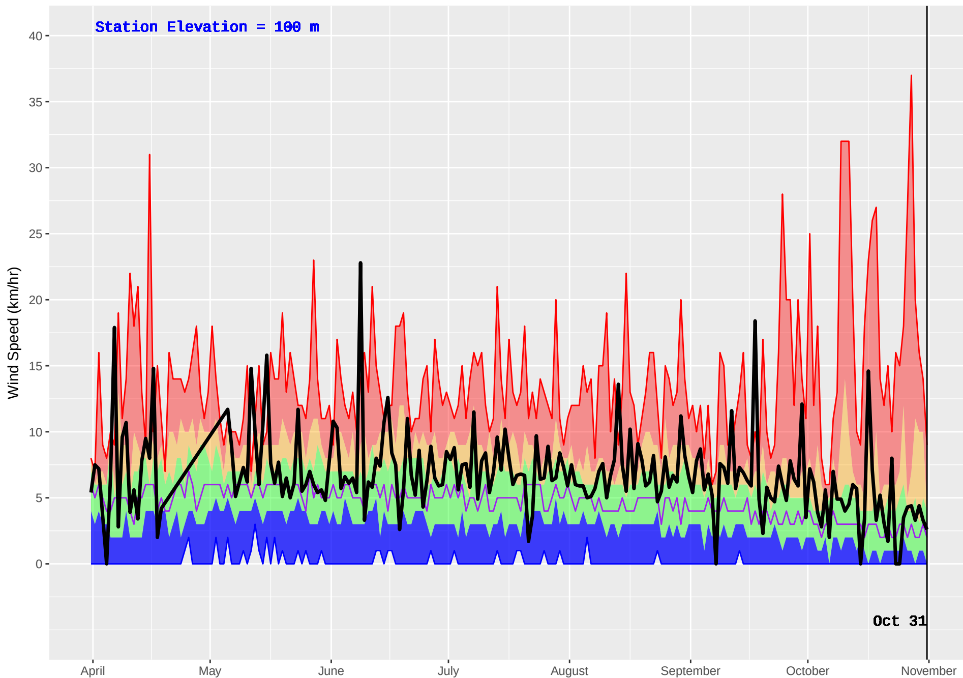
BEAVER CREEK (37) : Historical (1987–2016) and Current (2017) Noon Wind Speed
