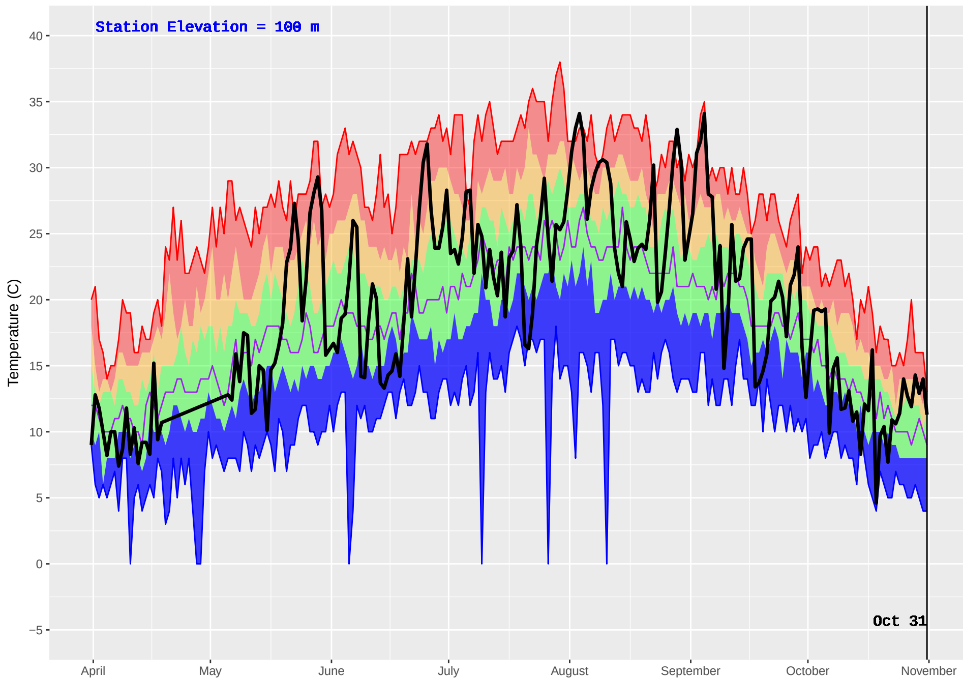
BEAVER CREEK (37) : Historical (1987–2016) and Current (2017) Noon Temperature
